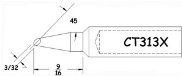
Conical Bevel
