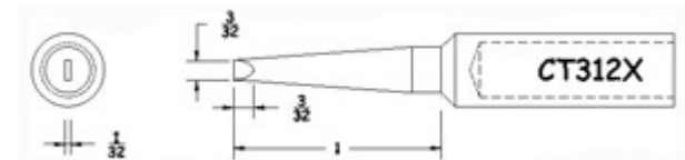
Full Chisel
