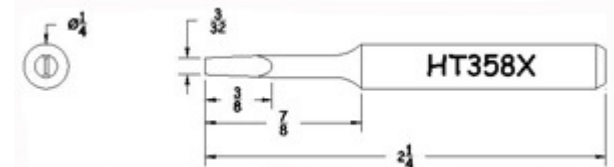
TD Semi-Chisel
