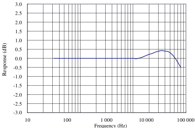
Fig. 2 Frequency response of the microphone UC-52
