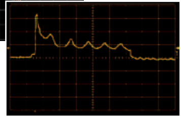
Automobile Starter Current 100 A/div 1 s/div
