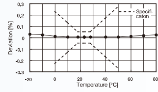
Sensitivity - Temperature Characteristics (9709)
