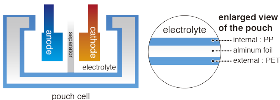
Figure 16. Example diagram of the structure of a laminated lithium-ion battery
