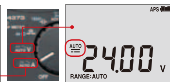
Voltage measurement
