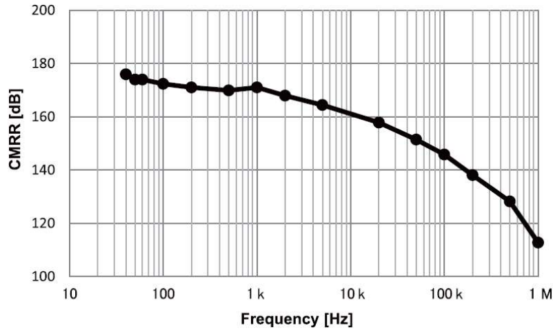
Figure 4. CMRR characteristics
