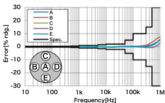
Fig. 5: Gain-frequency characteristics.
