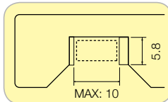
SMD TEST FIXTURE 9677
