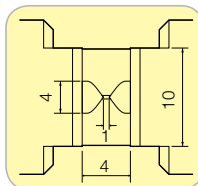
PINCHER PROBE 9143-10
