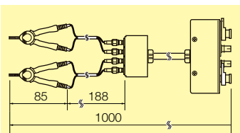
FOUR-TERMINAL PROBE L2000
