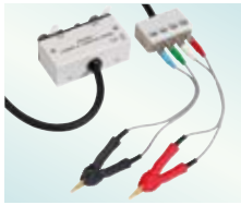
FOUR-TERMINAL PROBE L2000
