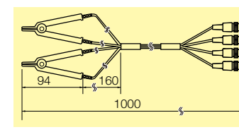
FOUR-TERMINAL PROBE 9140-10
