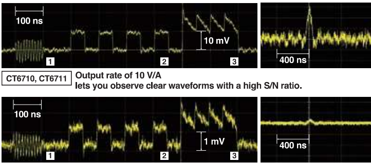
Earlier model Output rate of 1 V/A precludes observation of accurate waveforms as they are obscured by noise.
