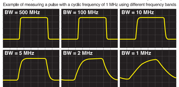
Current probes with a wide frequency band can accurately capture pulse waveforms.
