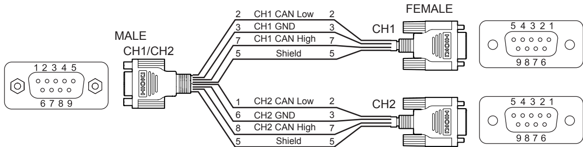
Pin assignments
