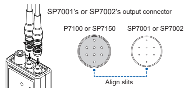
Example: SP7100 CAN Interface
