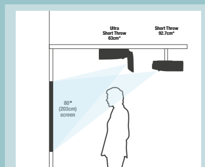
Short Throw distance diagram
