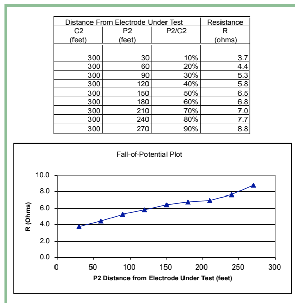
Figure 6: Earth impedance can be found from this curve by using the Tagg Slope Technique
