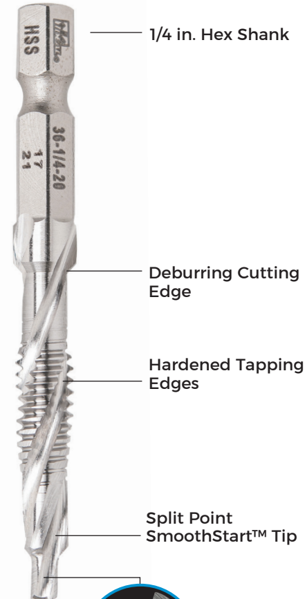
3-flute Design
