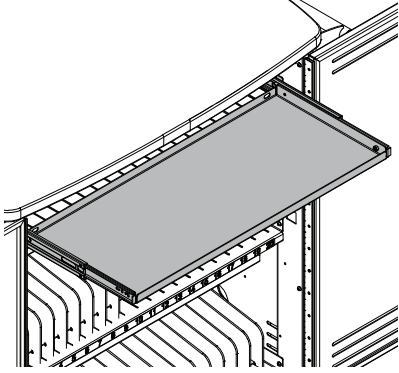
Pull-out Instructor Shelf (for instructor laptop or storage) 25 \frac{7}{16} "W x 11 \frac{3}{8} "D x 3 \frac{13}{16} "H 55442
