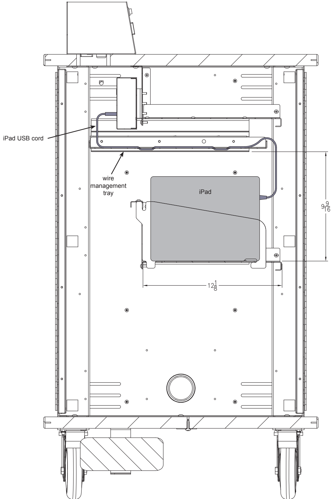
InTouch 20 Cart section view
