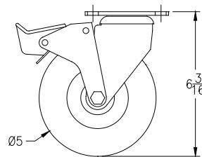
5" balloon wheel
