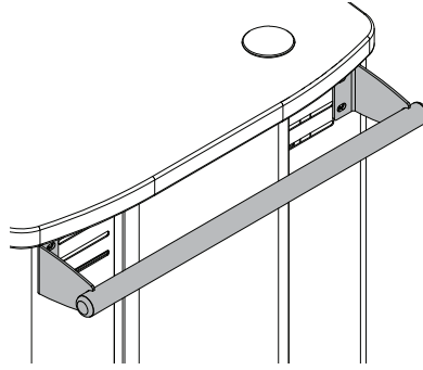
Additional Steel Handle (mounts on left or right-max 2 per unit) 20 \frac{3}{16} "W 55393
