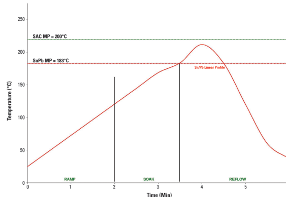
SnPb Reflow Profile
