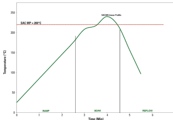
SAC Alloy Reflow Profile
