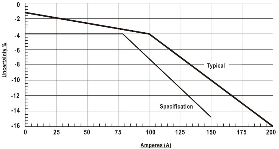
Figure 8. DC signal linearity in the 20 mV/A range, typical
