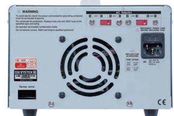
Rear Panel
