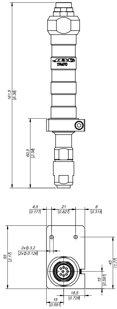
Soldering Iron Ref. TR470-B
