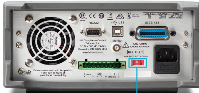
AC line voltage indicator
