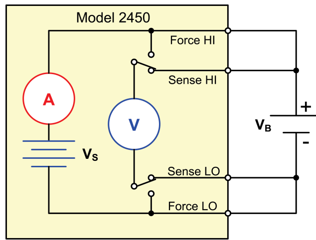
Figure 42: Schematic for the battery charge and discharge cycle test
