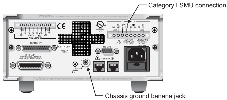
Figure 2 Typical instrument connector
