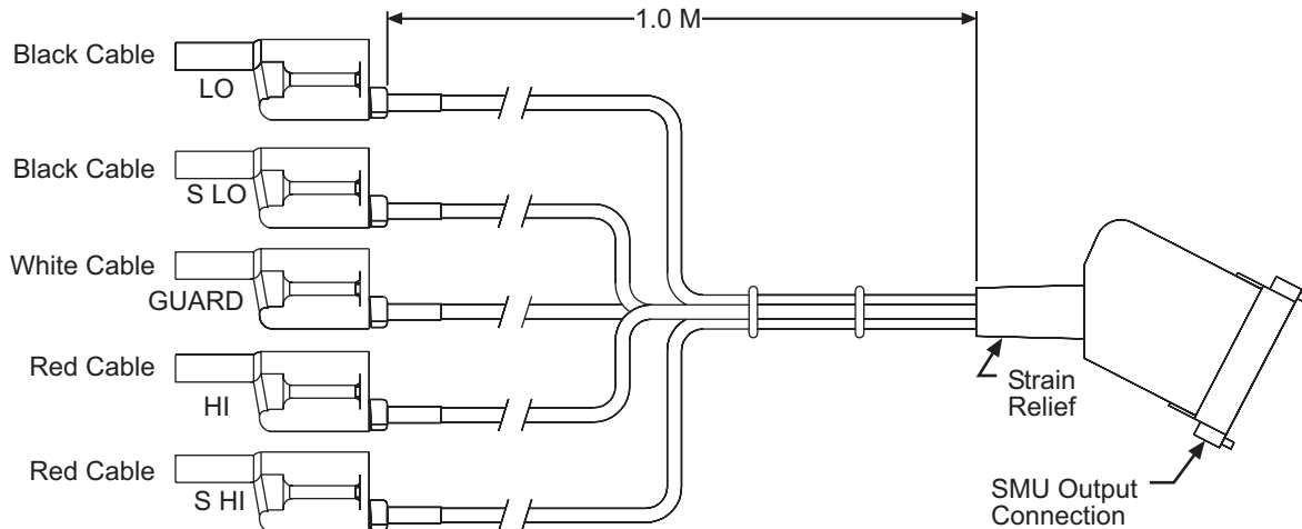
Figure 1 Cable features
