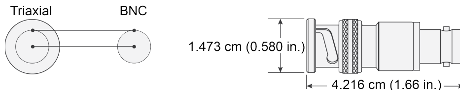
Figure 2: 7078-TRX-BNC (CS-633) adapter dimensions
