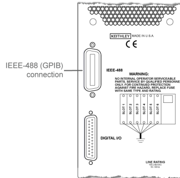
Figure 8: Model 707B rear panel IEEE-488 connection
