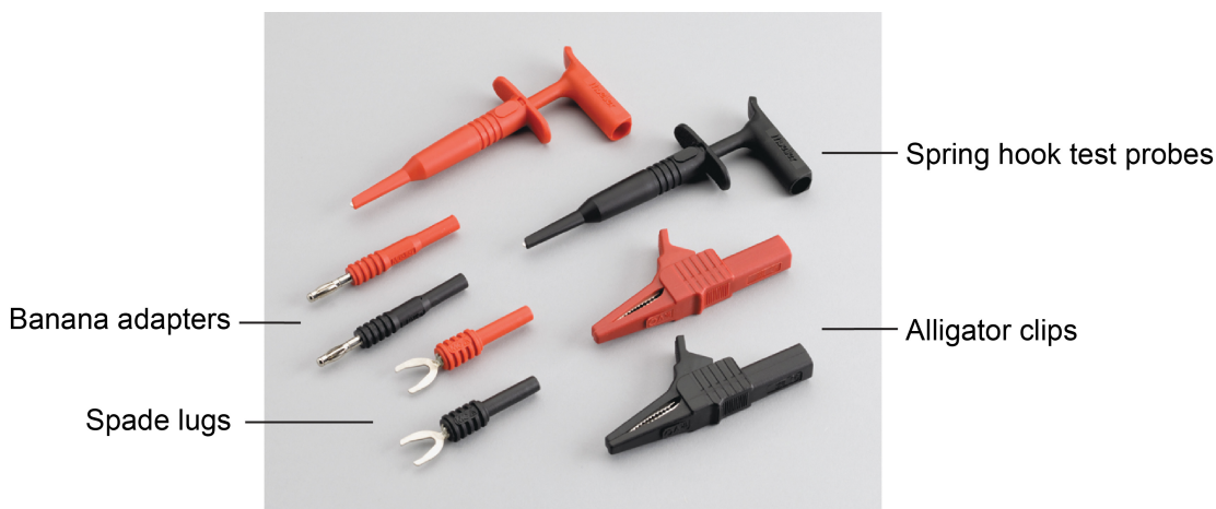
Figure 1: Model 8606 High Performance Probe Tip Kit
