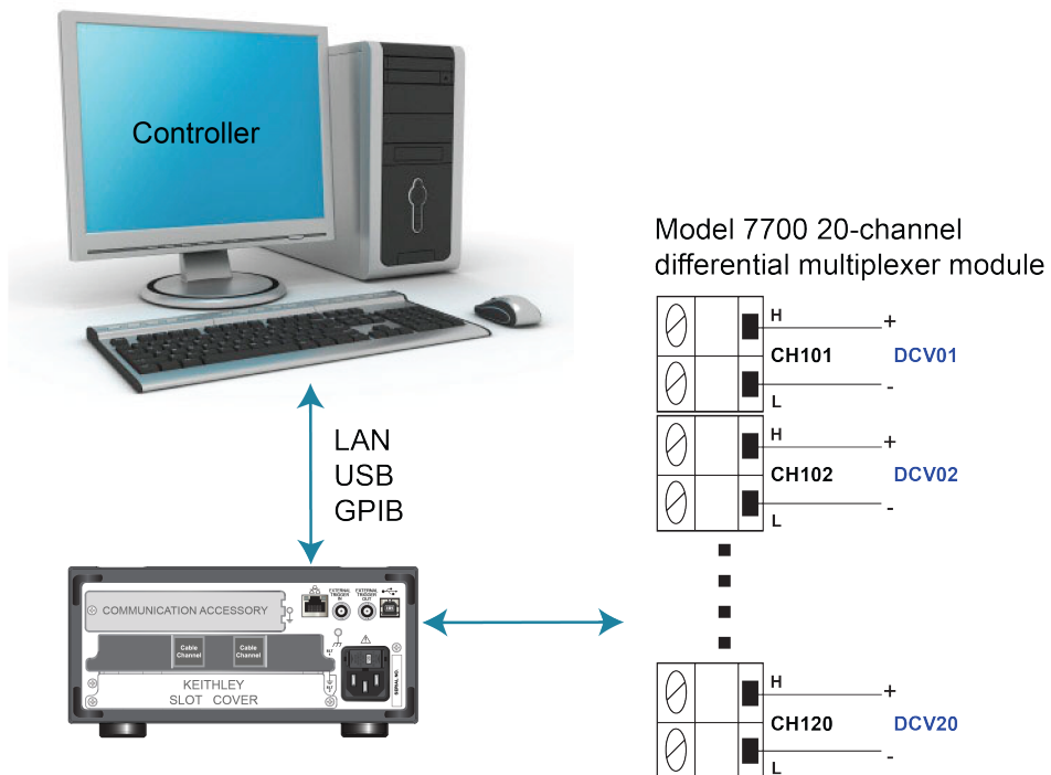
Figure 44: DAQ6510 speed scanning instrument and device connection
