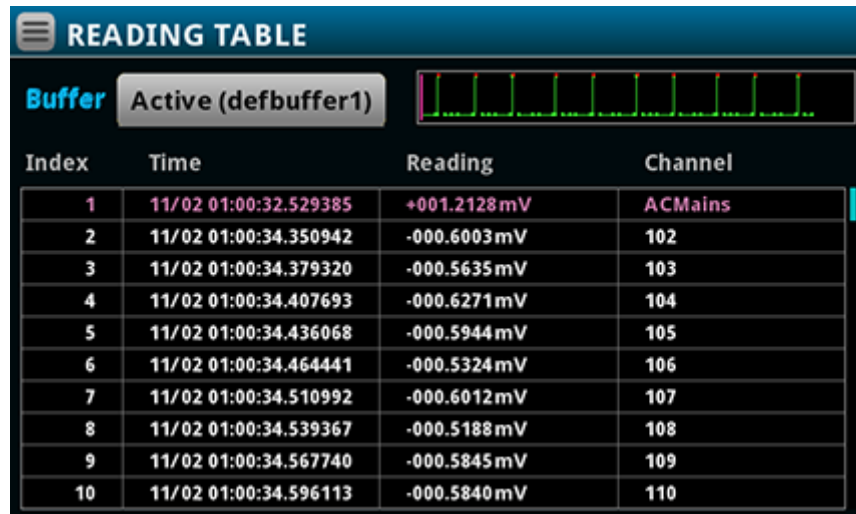
Figure 43: DAQ6510 reading table mixed function multichannel scanning
