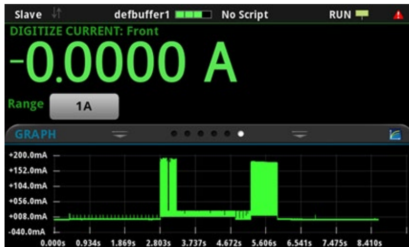
Figure 48: Subordinate node current waveform
