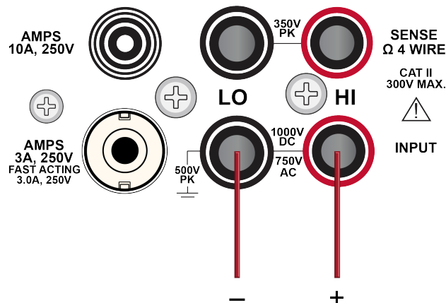
Figure 33: Rear-panel connections
