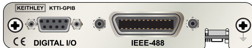
Figure 21: KTTI-GPIB connector view
