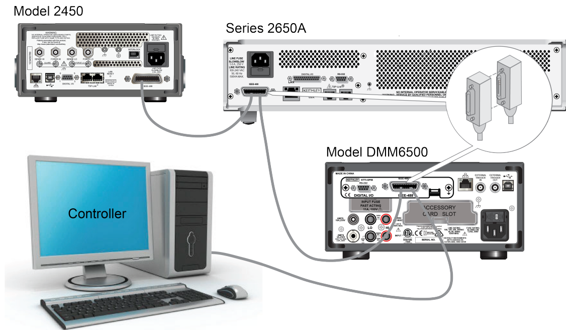
Figure 23: DMM6500 instrument GPIB connections
