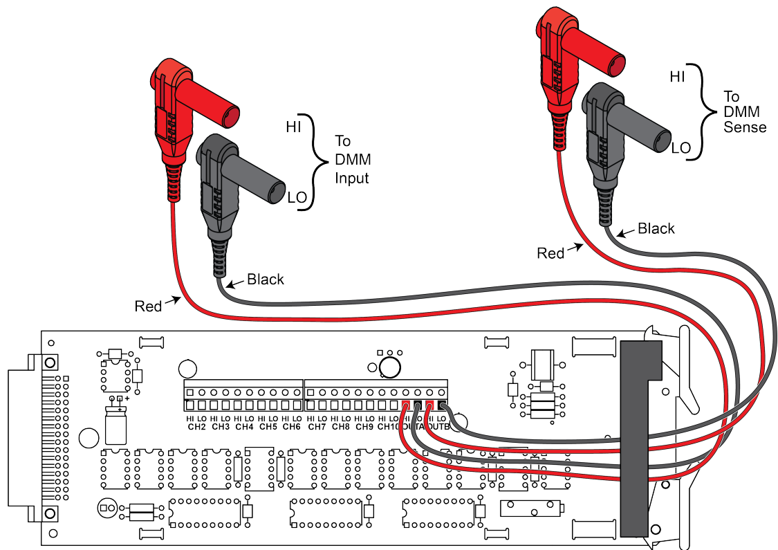
Figure 38: 2001-TCSCAN card
