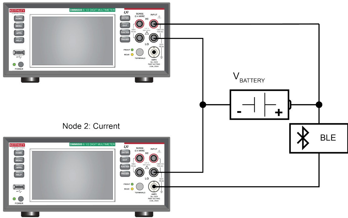
Figure 44: Two nodes measuring current and voltage
