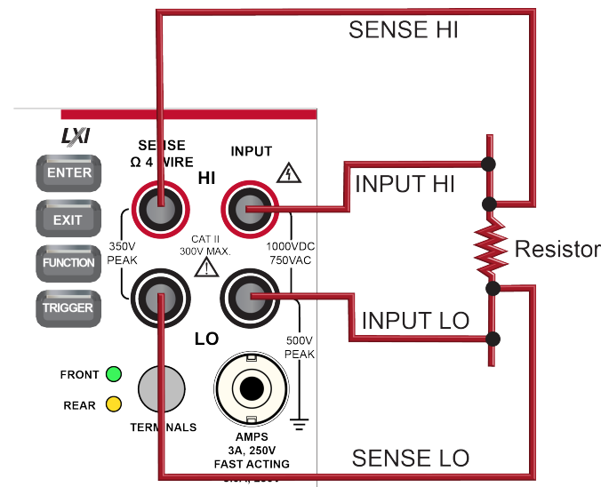
Figure 35: Front-panel connections for 4-wire resistance measurements
