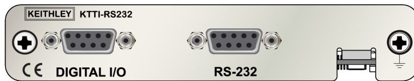
Figure 26: RS-232 panel connector
