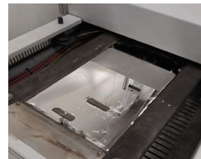
Solder pot post cleaning. Shiny with no evidence of dross.
