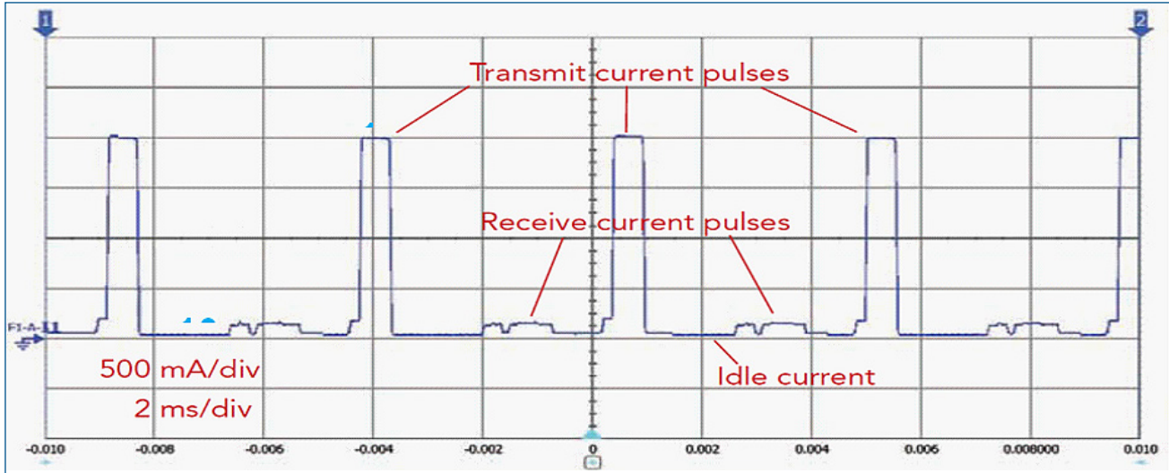
Figure 1 The current drain measured on a GSM cell phone when making a call.
