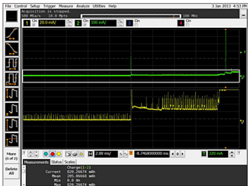
Figure 5 Keysight's Infiniium and InfiniiVision oscilloscopes provide an area under the curve measurement (Charge), where you can easily calculate the integrated current consumptions in Ah (Ampere x Hour) over time.
