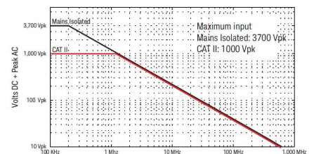
10076C derating curve
