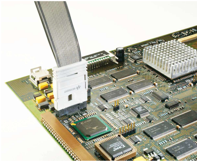
E5346A 34-channel Mictor connector probe
