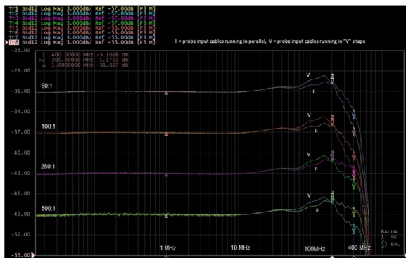
Frequency response of DP0001A
