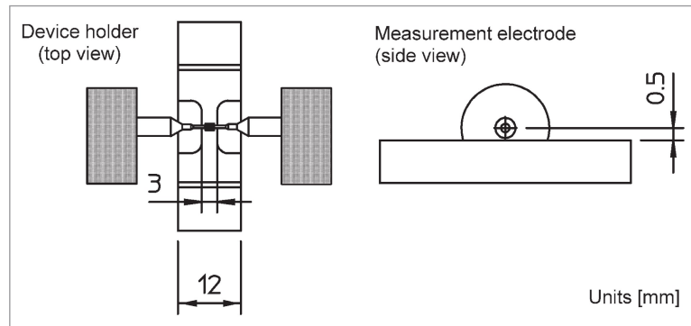
Electrode dimensions
