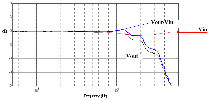
Figure 136 Graph of Vin and Vout of probe with a 25Ω source and Vout/Vin frequency response.
