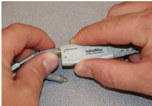
Figure 4 Properly Pulling the Probe Head Straight Out
