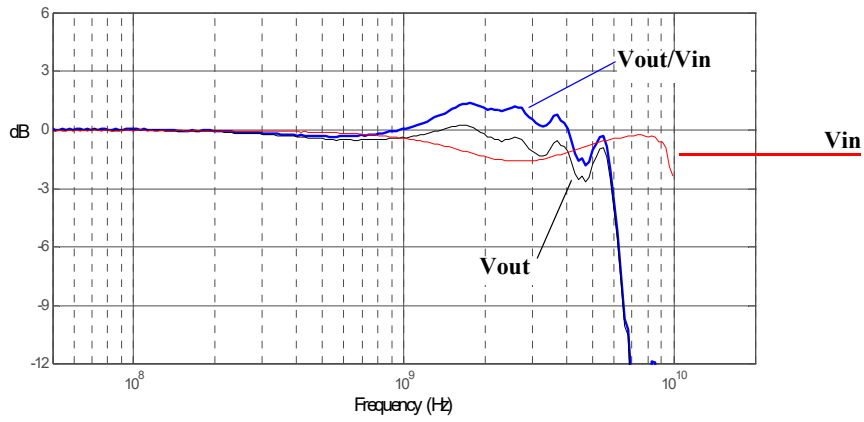
Figure 147 Graph of Vin and Vout of probe with a 25Ω source and Vout/Vin frequency response.
