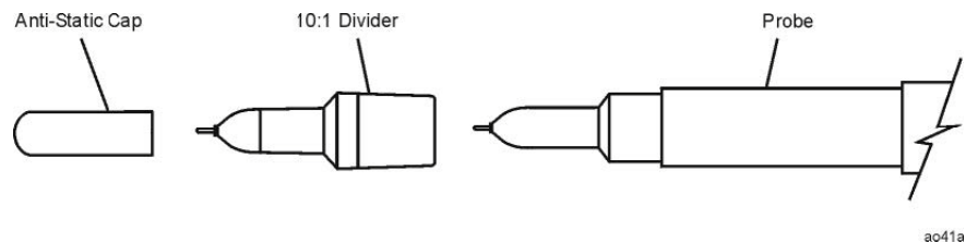
Figure 1-1 Probe with 10:1 divider and anti-static protection cap
