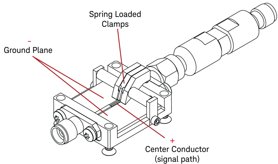
Figure 13 Signal Path and Ground Locations on PV Fixture
