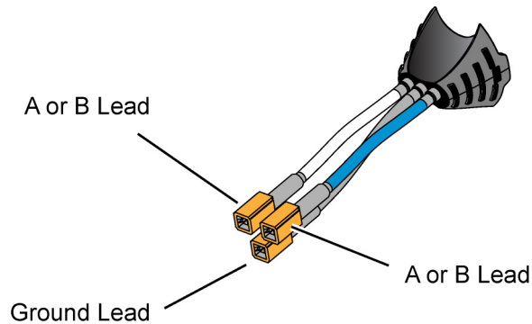
Figure 7 Socketed Tip
