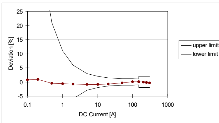
Figure 16 DC Accuracy Characteristic N2781B
