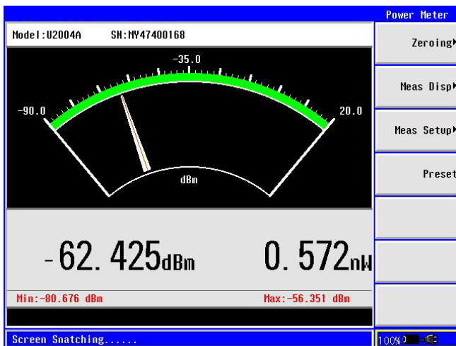
Figure 14. N9340B HSA HSA turns into a power-meter measurement
