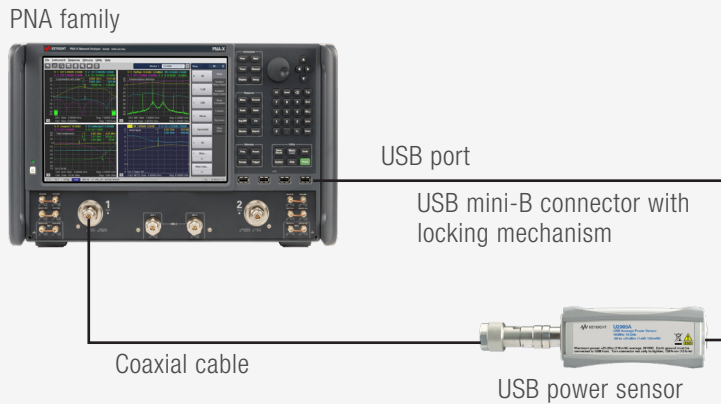
Figure 3. USB power sensor connecting directly to a PNA USB port through a USB mini-B connector.
