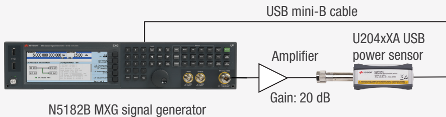
Figure 23. Power meter servo configuration
