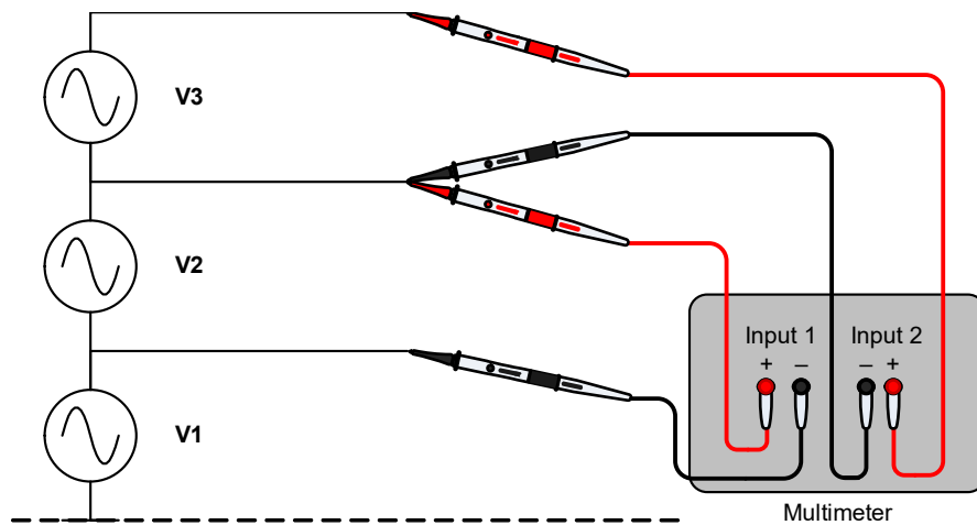
Figure 1-6 Ground loop
