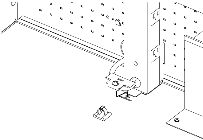
DETAIL 'C'
