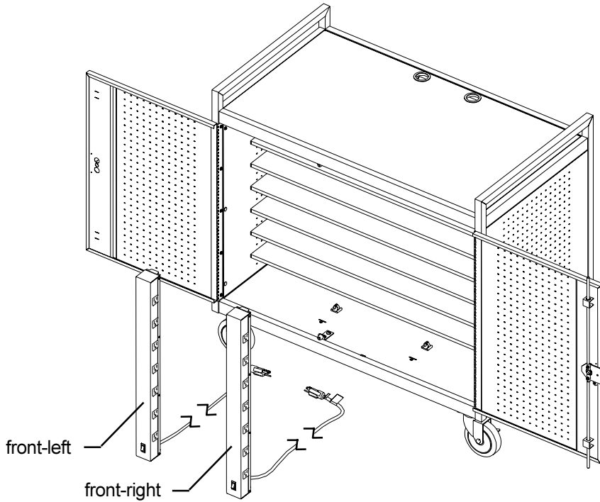
DETAIL 'A'
