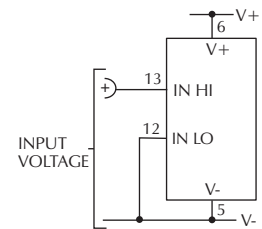
Check Links 1, 3 & 4 are SHORTED. Measuring a single ended input referenced to supply (DPM 160S).
