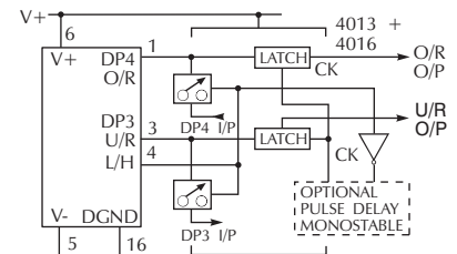
Check Link REF is SHORT. Driving DP3 and DP4 inputs while monitoring under range and over range outputs.
