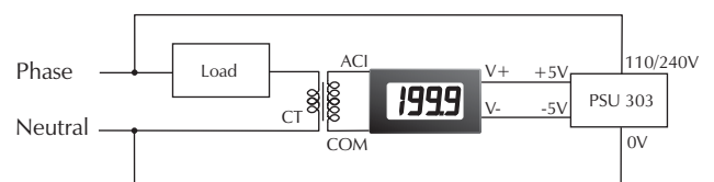
Using a current transformer (CT) to measure currents in excess of 10A a.c.
