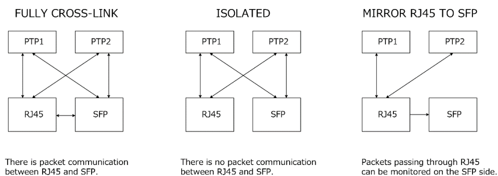
Figure 21-1 PORT RELATION
