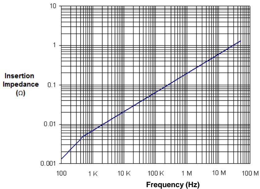
Figure 4. Insertion impedance vs. frequency.
