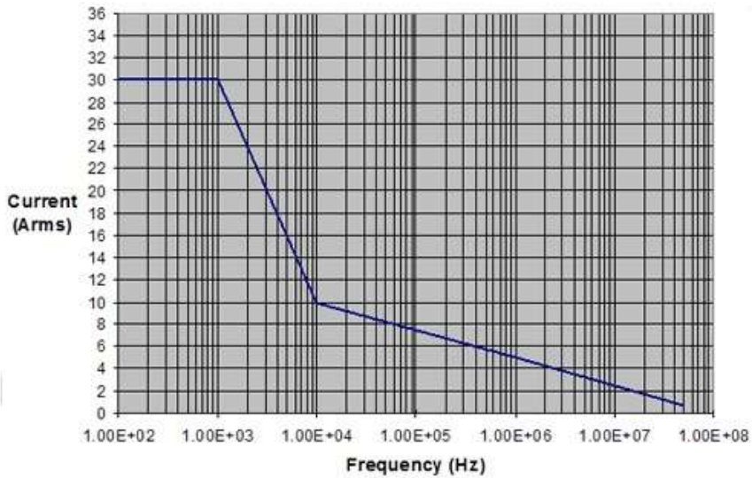
Figure 3. Maximum input current vs. frequency.
