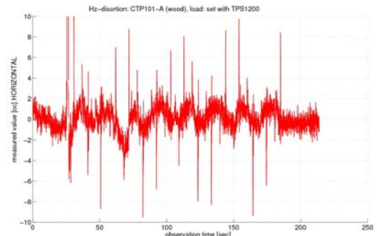
Figure 5b - Leica GST101 wood tripod
