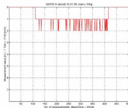
Figure 4a - Leica GST05 tripod
