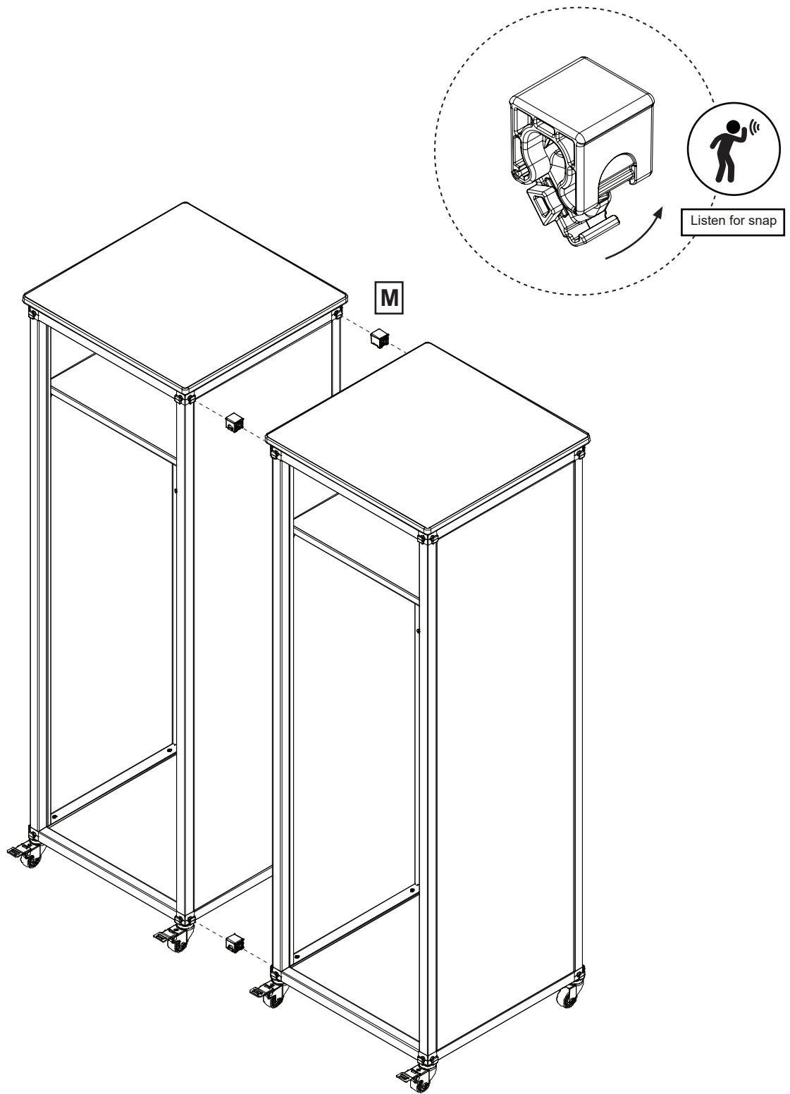
Example of MBSCB05 connected horizontally
