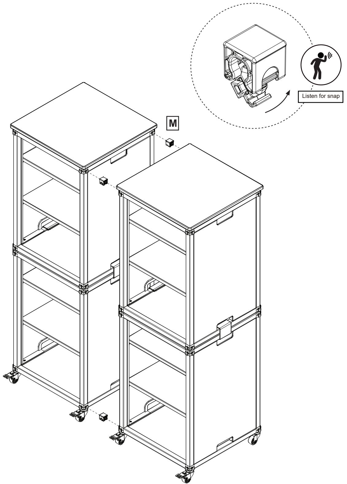
Example of MBSCB06 connected horizontally
