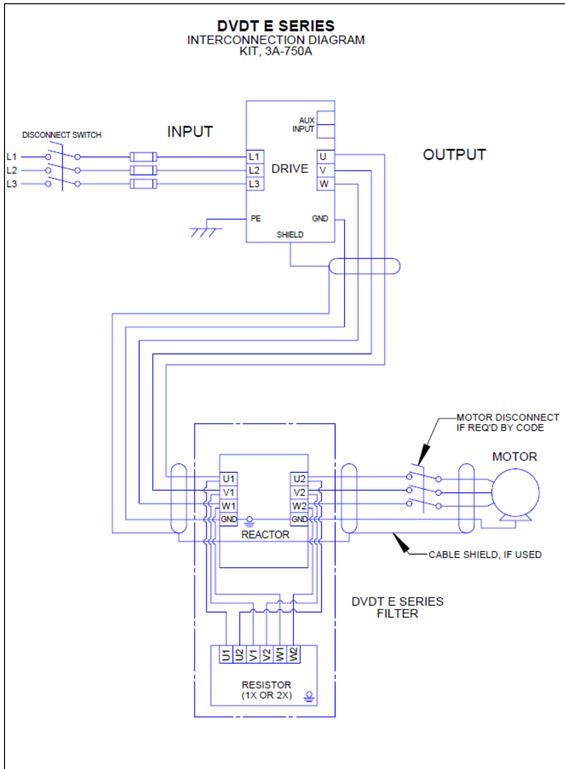
Figure 5-2: Kit Diagram
