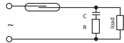
Diagram C: RC Network
