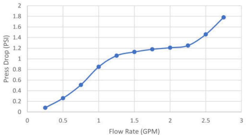
Pressure Drop vs. Flow Rate
