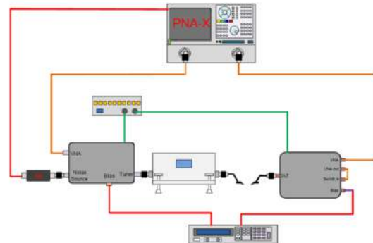
Figure 2. Block diagram of typical Noise Parameters setup with combined VNA and NFA
